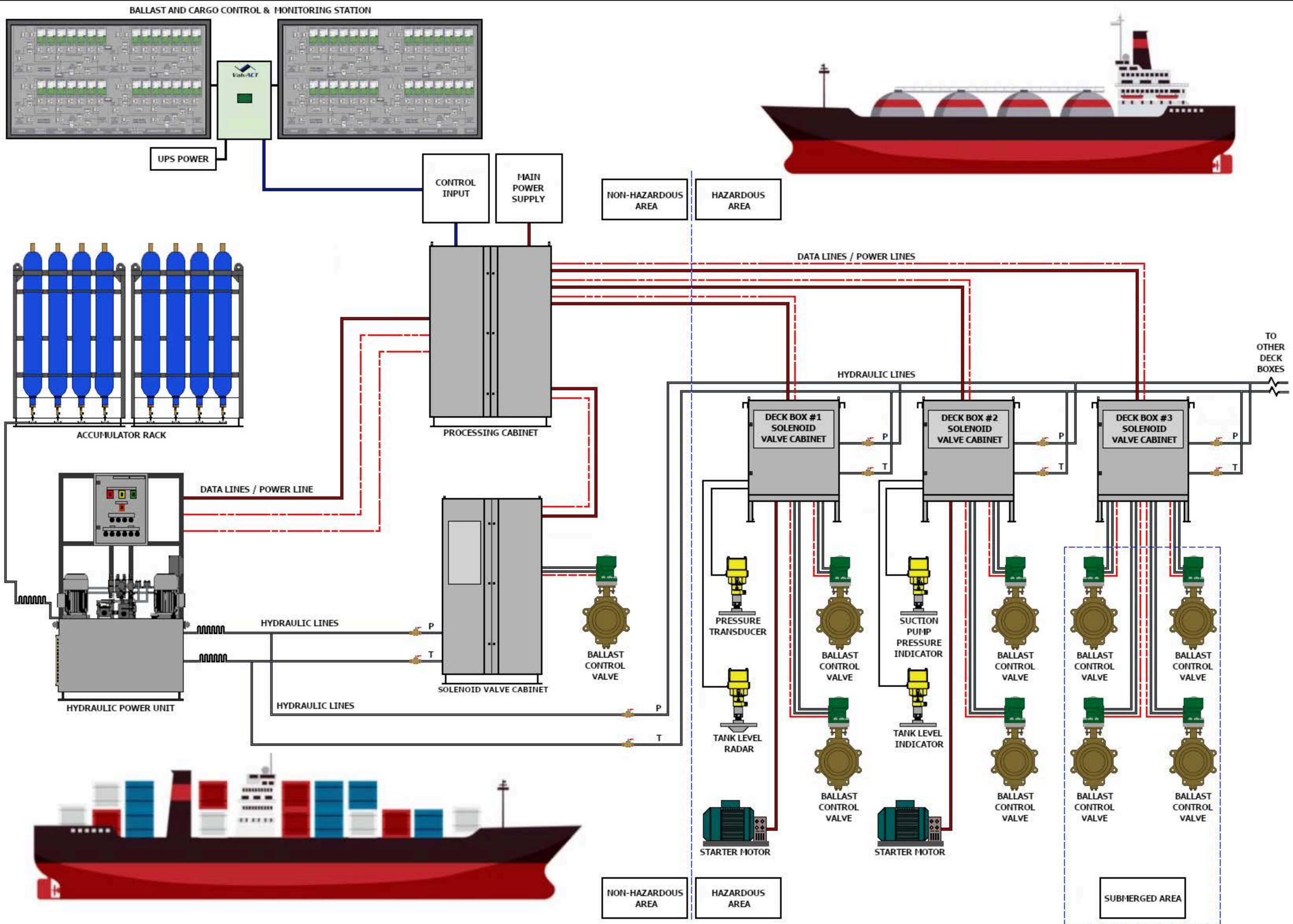
ValvACT Conventional Hydraulic Ballast Control System
