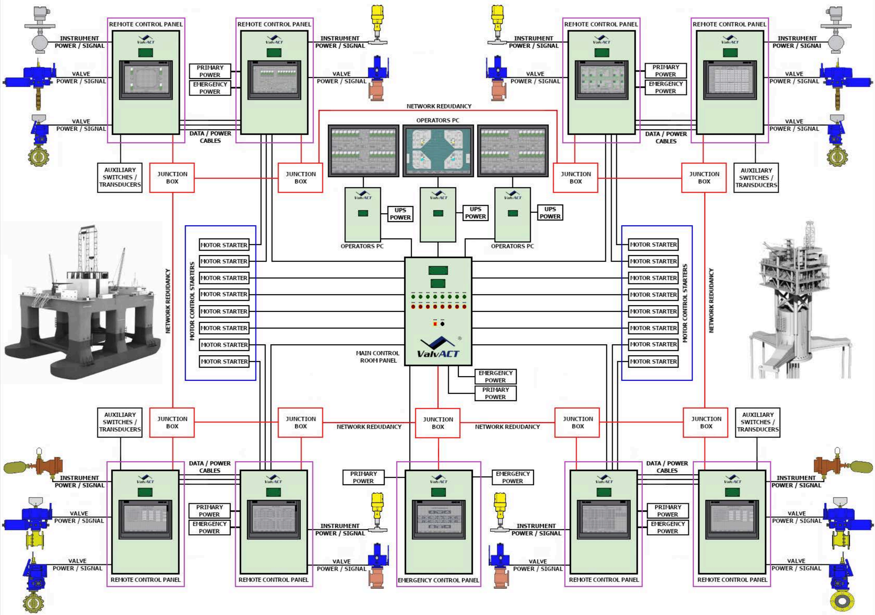
ValvACT, Inc. Electro-Hydraulic Ballast Control System
